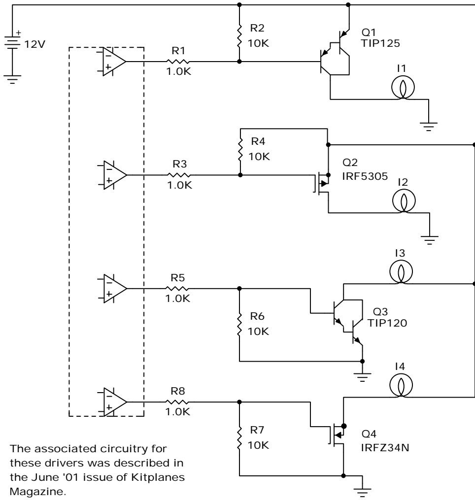
Case 1: Power-switched PNP bipolar design.
